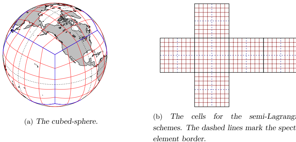
Figure 1.5. The figure (a) shows the cubed-sphere whereas in (b) the finite volume grid on the spectral element grid (dashed lines) on the cube faces is visualized. This grid results of a gnomonic projection of the sphere. The cells are not equidistantly spaced as it is shown here for the sake of simplicity.
